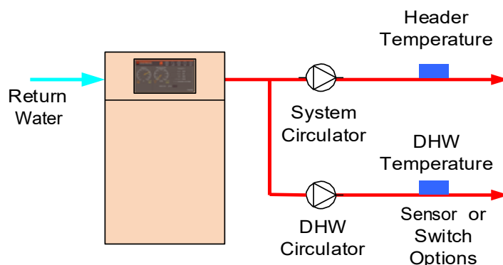
Figure 7: Single Unit Hydronic Options
