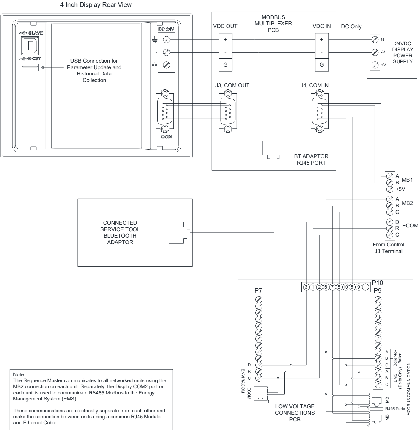
Figure 14a: Display Terminal Layout and wiring notes
