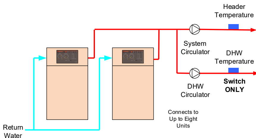
Figure 8: Multiple Unit Hydronic Options
